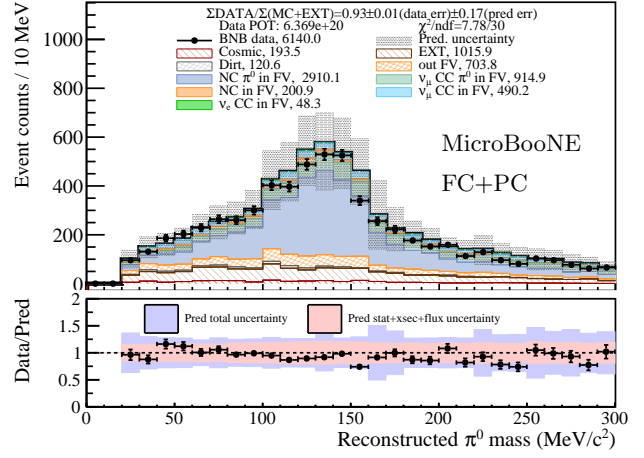
(b) NC\pi^0 reconstructed \pi^0 mass
