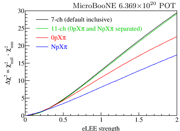
FIG. 32: \Delta\chi_{\text{nested}}^2 value as a function of eLEE strength. “7-ch” (black curve) corresponds to the result from the default 7-channel simultaneous fit which is the same as the one in Fig. 28. “11-ch” (green curve) corresponds to the result from a 11-channel simultaneous fit combining separated 0pX\pi and NpX\pi channels for \nu_e CC and \nu_\mu CC FC and PC events together with the dedicated \pi^0 channels. “ 0pX\pi ” (red curve) corresponds to the result from the 0pX\pi channels for \nu_e CC and \nu_\mu CC FC and PC events as well as the dedicated \pi^0 channels. “ NpX\pi ” (blue curve) corresponds to the result from the NpX\pi channels for \nu_e CC and \nu_\mu CC FC and PC events as well as the dedicated \pi^0 channels.
