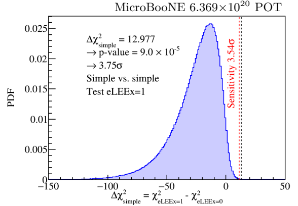
(b) eLEE_{x=1} hypothesis.
