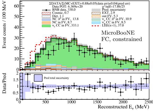
FIG. 25: Event distribution of FC \nu_e CC candidates as a function reconstructed E_\nu . Same set-up as that of Fig. 24 except that the constraint from PC \nu_e CC, FC \nu_\mu CC, PC \nu_\mu CC, FC CC\pi^0 , PC CC\pi^0 , and NC \pi^0 is used.
