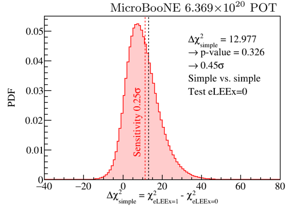
(a) eLEE_{x=0} hypothesis.
