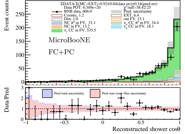
(b) Shower \cos\theta , broken down with event types
