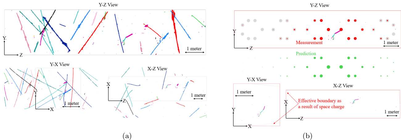
FIG. 4: A \nu_e CC interaction candidate from MicroBooNE data. The X axis is the drift electric field direction from the TPC anode to the cathode. The Y axis is vertical up, and the Z axis is along the neutrino beam direction. Panel (a) shows three 2D projections of reconstructed 3D clusters in the full TPC readout window before charge-light matching. Each cluster is shown in a different color. The gray box represents the TPC active volume while the two ends along the X axis correspond to the trigger time and the maximum drift time relative to the trigger. Panel (b) shows the 2D projections of the \nu_e CC candidate cluster after applying the charge-light matching. The red (green) circles represent the observed (predicted) number of photoelectrons (PEs) at each PMT, where the area of the circle is proportional to the number of PEs. The effective detector boundary as a result of the space charge effect is indicated by the red dashed lines in the corner of the TPC active volume as shown in the “Y-X view” and “X-Z view”.
