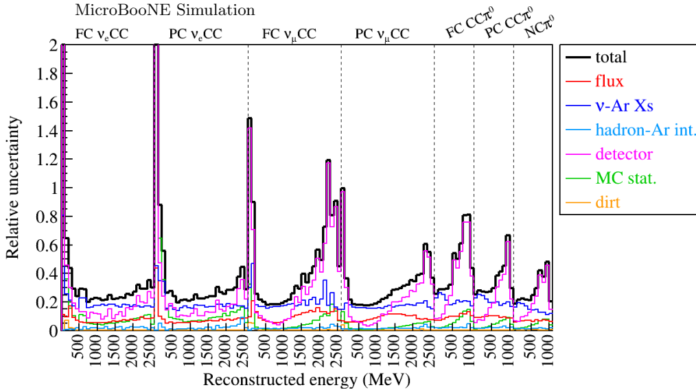
FIG. 12: Summary of relative uncertainties ( \frac{\text{absolute error}}{\text{prediction}} ) of all systematic uncertainty sources for the seven channels. Spikes at very low or high energy regions for detector systematic uncertainty are largely attributed to statistical errors stemming from the finite size of related MC samples.
