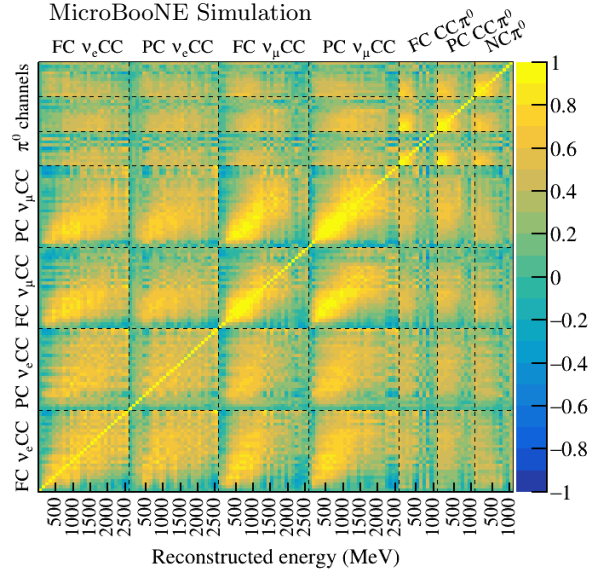
FIG. 19: Correlations of all systematic uncertainties for the seven channels.
