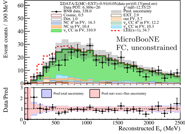
(a) \nu_e CC fully contained events.
