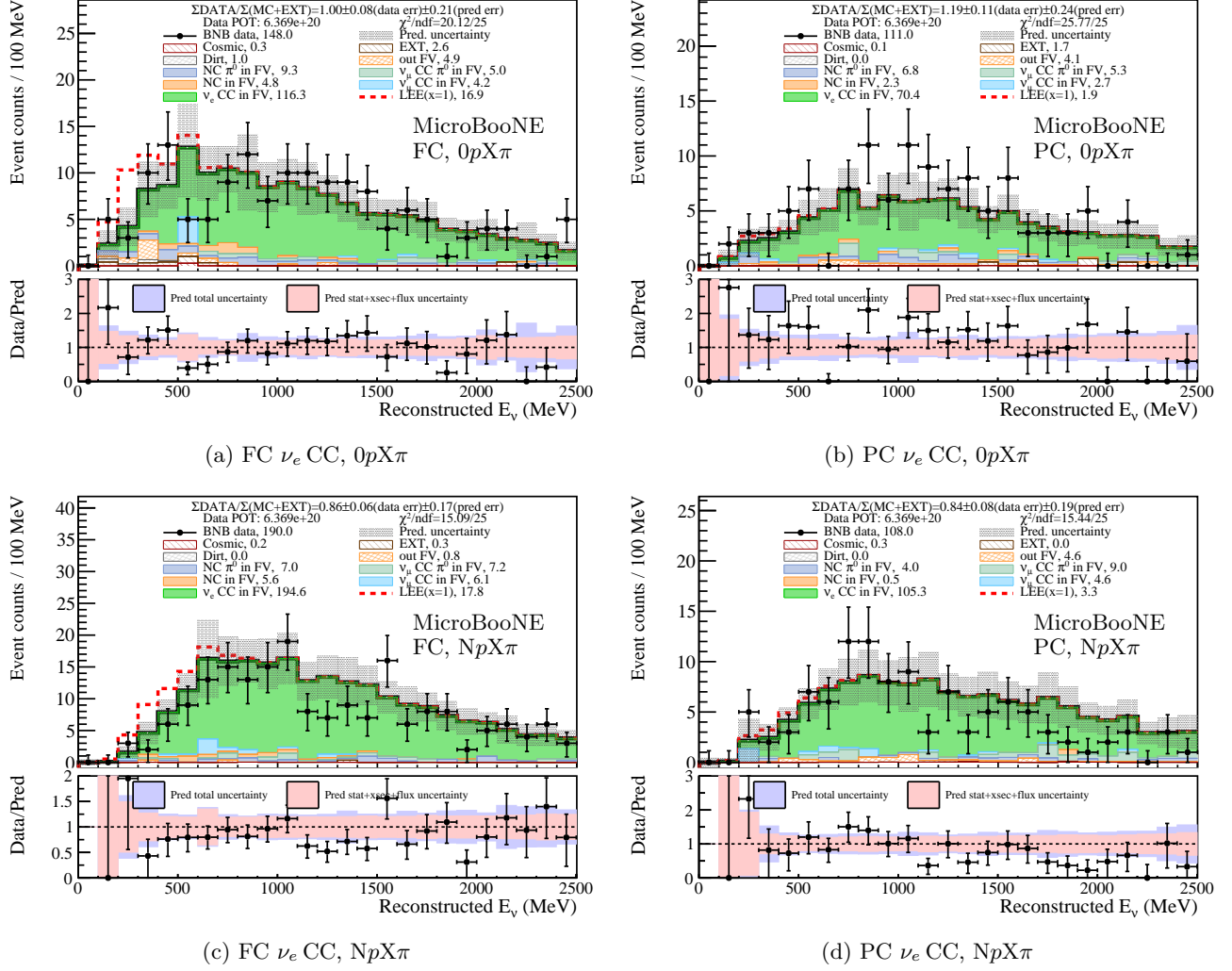
FIG. 31: Event distributions of FC \nu_e CC 0pX\pi , PC \nu_e CC 0pX\pi , FC \nu_e CC NpX\pi , and PC \nu_e CC NpX\pi samples in figures (a)-(d), respectively. The breakdown of each component for different final states for both signal and background events is shown in the legend (see definitions in Sec. IV A). The bottom sub-panels present the data-prediction ratios as well as the statistical and systematic uncertainties. The pink band includes the MC statistical, cross section, and flux uncertainties. The purple band corresponds to the full uncertainty with an addition of detector systematic uncertainty. No constraint is applied.
