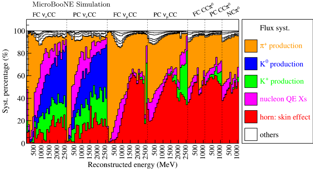
FIG. 13: Fraction ( \frac{\sigma_{\text{flux}}^2}{\sigma_{\text{flux}}^2} \times 100 ) of uncertainties of total flux systematics for the seven channels.
