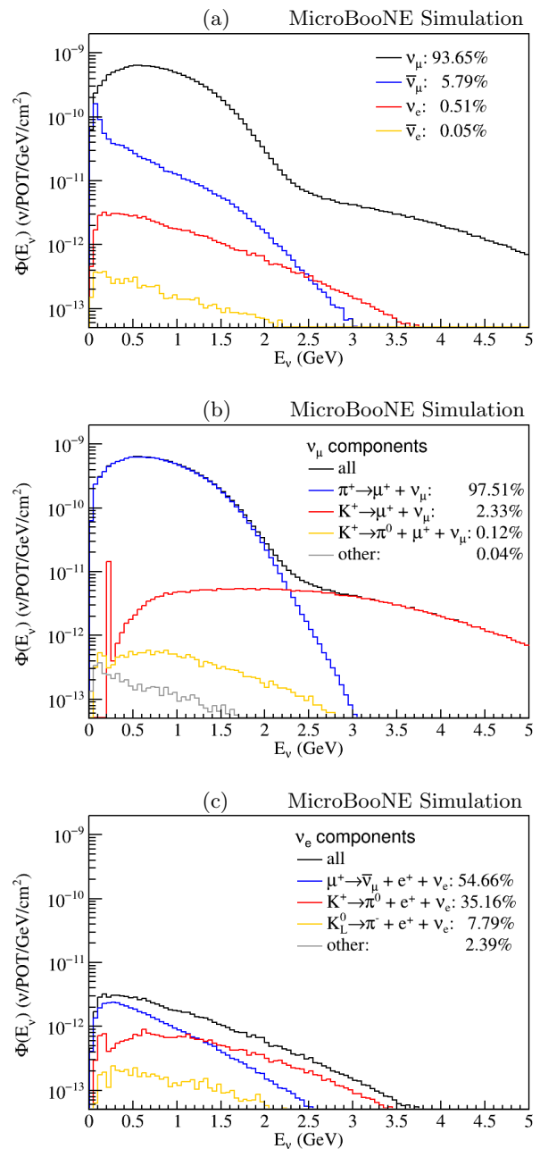
FIG. 2: Predicted neutrino flux from different decay modes at the MicroBooNE detector: (a) flux of different neutrino flavors, (b) \nu_\mu flux of different decay modes (the peak at 236 MeV corresponds to Kaon decay at rest), (c) \nu_e flux of different decay modes.
