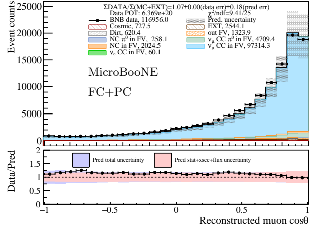
(b) Muon \cos\theta , broken down with event types
