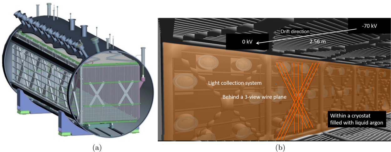
FIG. 3: Taken from Ref. [46]. (a) The MicroBooNE detector cryostat with the field cage shown inside. (b) Inside the cryostat of the MicroBooNE detector, visualized with the VENU software [50]. The maximum drift distance is 2.56 m with a drift electric field of 273 V/cm. The light-collection system, which consists of 32 PMTs, is located behind the three anode wire planes, which detect ionization charge.
