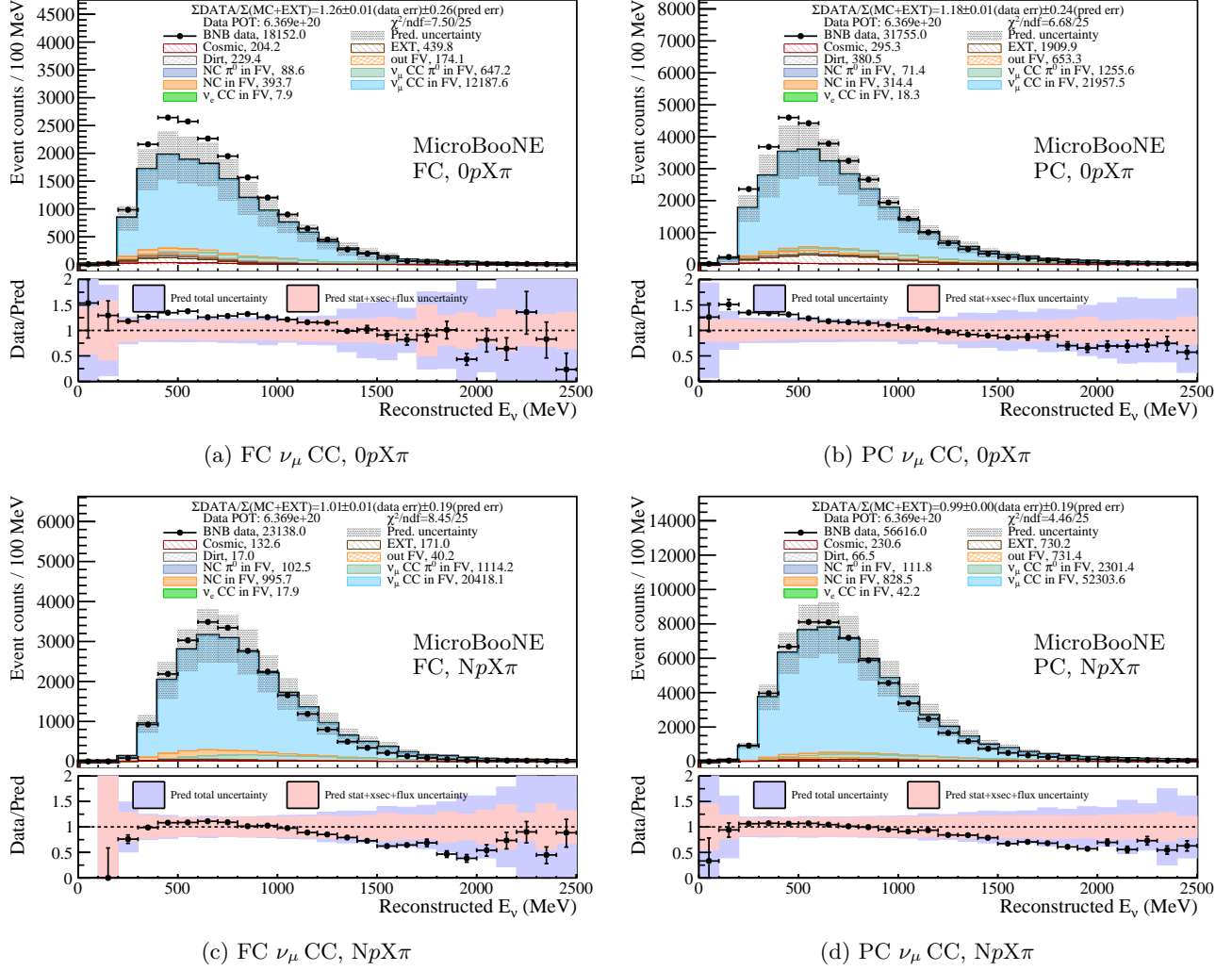
FIG. 30: Event distributions of FC \nu_\mu CC 0pX\pi , PC \nu_\mu CC 0pX\pi , FC \nu_\mu CC NpX\pi , and PC \nu_\mu CC NpX\pi samples in figures (a)-(d), respectively. The breakdown of each component for different final states for both signal and background events is shown in the legend (see definitions in Sec. IV A). The bottom sub-panels present the data-prediction ratios as well as the statistical and systematic uncertainties. The pink band includes the MC statistical, cross section, and flux uncertainties. The purple band corresponds to the full uncertainty with an addition of detector systematic uncertainty. No constraint is applied.
