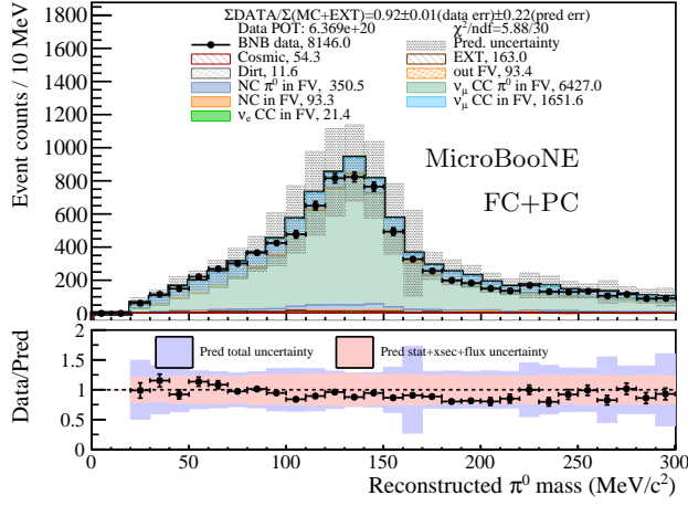
(a) CC\pi^0 reconstructed \pi^0 mass
