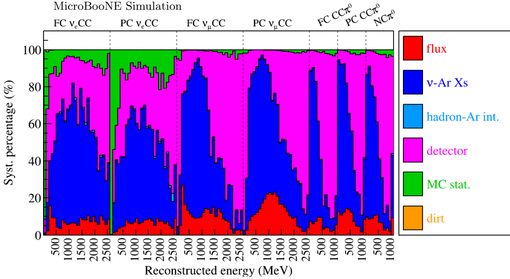
FIG. 20: Summary of fractional contributions to the overall systematic uncertainty ( \frac{\sigma_i^2}{\sigma_{\text{total}}^2} \times 100 ) for the seven channels.
