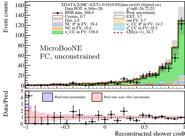
(c) \nu_e CC shower \cos\theta , fully contained events.
