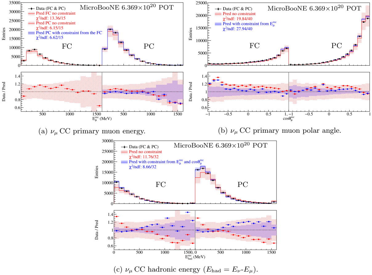
FIG. 22: Event distributions of reconstructed muon energy (a), muon angle (b), hadronic energy (c), for selected \nu_\mu CC events with fully contained (FC) events on the left half and partially contained (PC) events on the right half in each sub-figure. Black points are from data measurements. Red (blue) histograms and error bands are for the MC prediction before (after) constraint. The last bin is the overflow bin for FC or PC muon energy or hadronic energy distributions.
