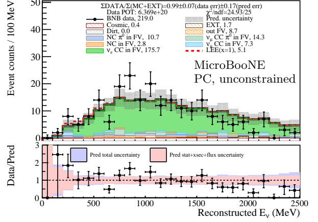
(b) \nu_e CC partially contained events.
