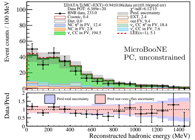
(f) \nu_e CC hadronic energy, partially contained events.
