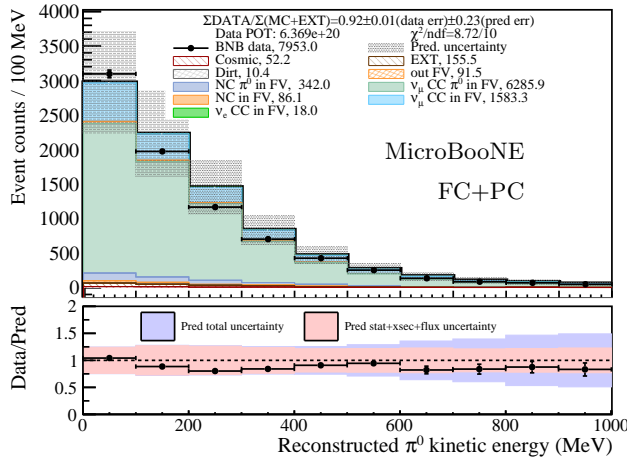
(c) CC\pi^0 reconstructed \pi^0 kinetic energy
