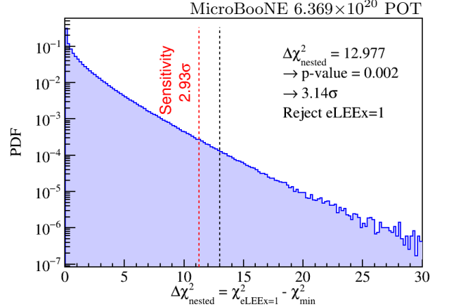
FIG. 29: Distribution of \Delta\chi^2_{\text{nested}} assuming \text{eLEE}_{x=1} is true. The sensitivity of rejecting the \text{eLEE}_{x=1} hypothesis is at 2.93\sigma following the Feldman-Cousins procedure. Using the same procedure, the data measurement rejects \text{eLEE}_{x=1} hypothesis at the p-value of 0.002, which corresponds to 3.14\sigma . The results are obtained from 10 million pseudo experiments.
