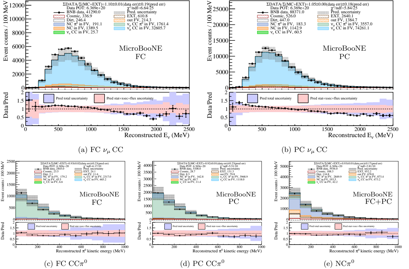
FIG. 21: Event distributions of FC \nu_\mu CC, PC \nu_\mu CC, FC CC\pi^0 , PC CC\pi^0 , and NC\pi^0 in (a)-(e), respectively. These five selections serve as constraints to reduce the systematic uncertainties in searching for eLEE, thus maximizing the physics sensitivity. The breakdown of each component for different final states for both signal and background events is shown in the legend. The bottom sub-panels present the data-to-prediction ratios as well as the statistical and systematic uncertainties. The pink band includes the statistical, cross section, and flux uncertainties. The purple band corresponds to the full uncertainty with an addition of detector systematic uncertainty.
