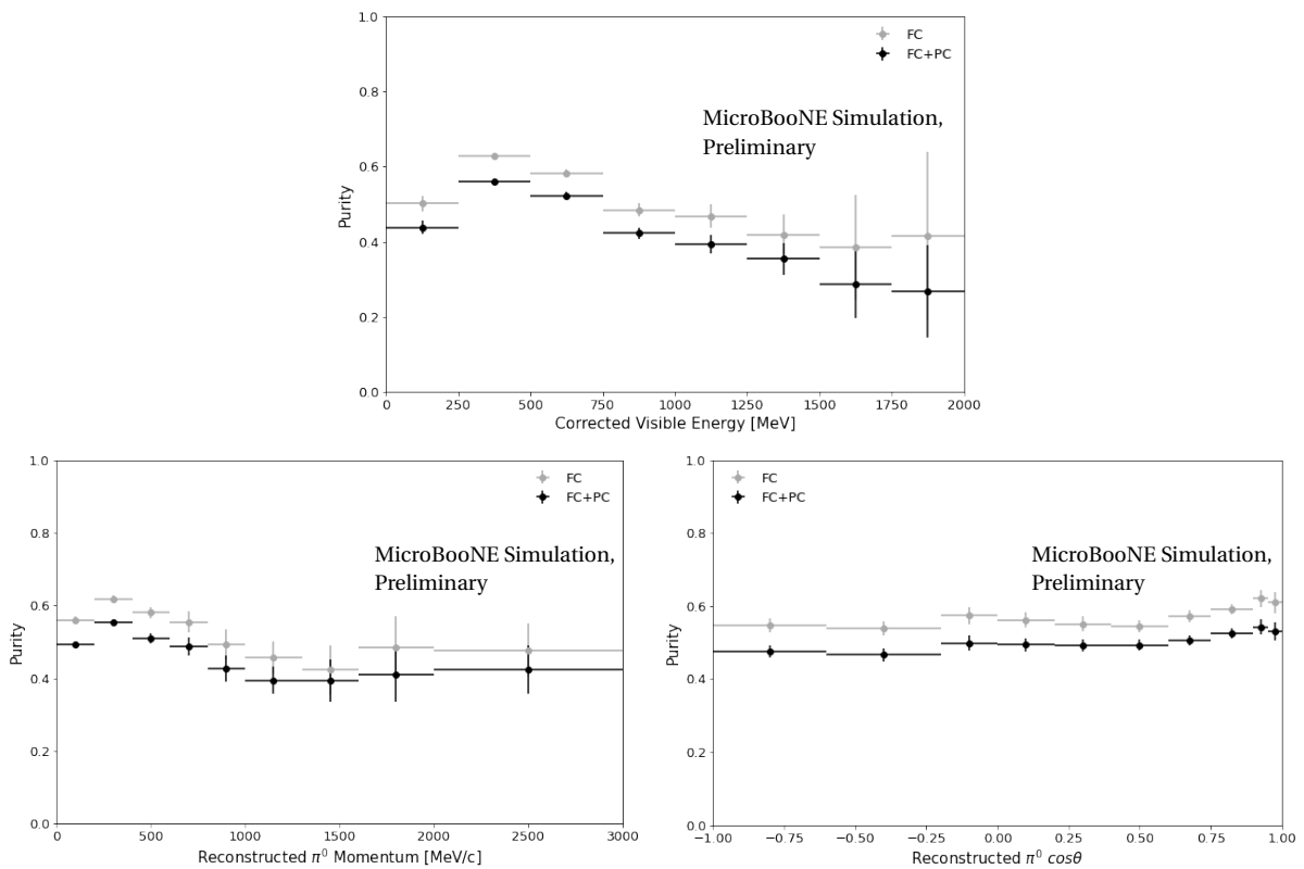
Figure 8: Purity for signal events as a function of the corrected visible energy (Top), reconstructed \pi^0 momentum (Bottom Left) and reconstructed \pi^0 angle (Bottom Right) for selected \text{NC}\pi^0 events.
