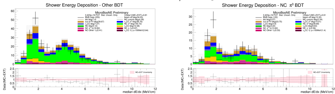
(c) The shower stem dE/dx after preselection and the \nu_\mu CC and other background BDT cuts. (d) The shower stem dE/dx after preselection and the \nu_\mu CC, other, and NC \pi^0 background BDT cuts.
