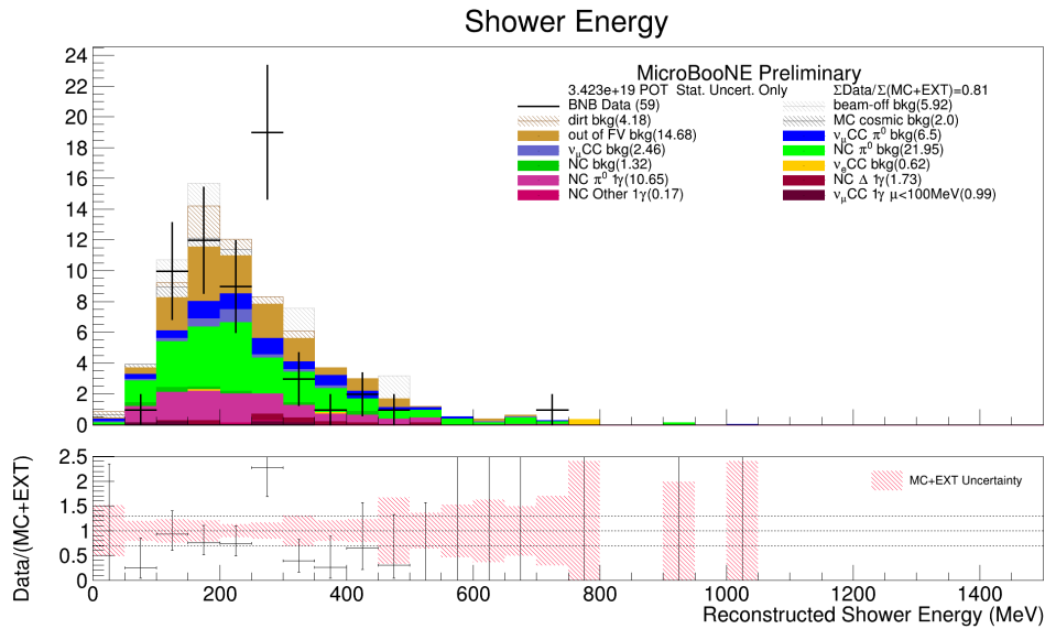
Figure 9: Reconstructed shower energy for selected events.
