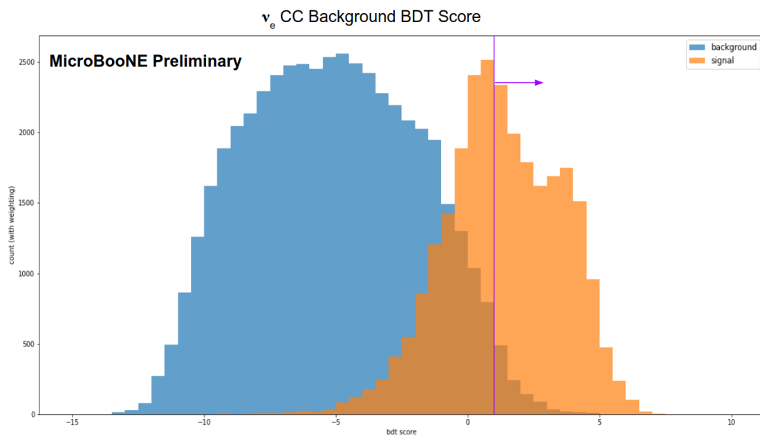
Figure 6: \nu_e CC background removal BDT scores. Background includes only \nu_e CC events from BNB overlay and \nu_e CC overlay. The purple line indicate the cut value for the selection.
