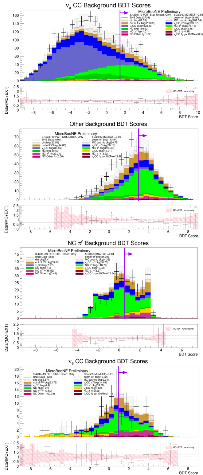
Figure 8: BDT score for each of the 4 BDTs, after preselection and relevant earlier BDT cuts. The purple line indicates the cut value.
