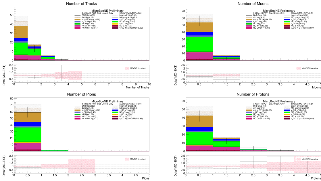
Figure 11: Number of reconstructed tracks and the breakdown of muon, charged pion, and proton tracks, determined by Wire-Cell’s particle flow and identification algorithms for selected events.
