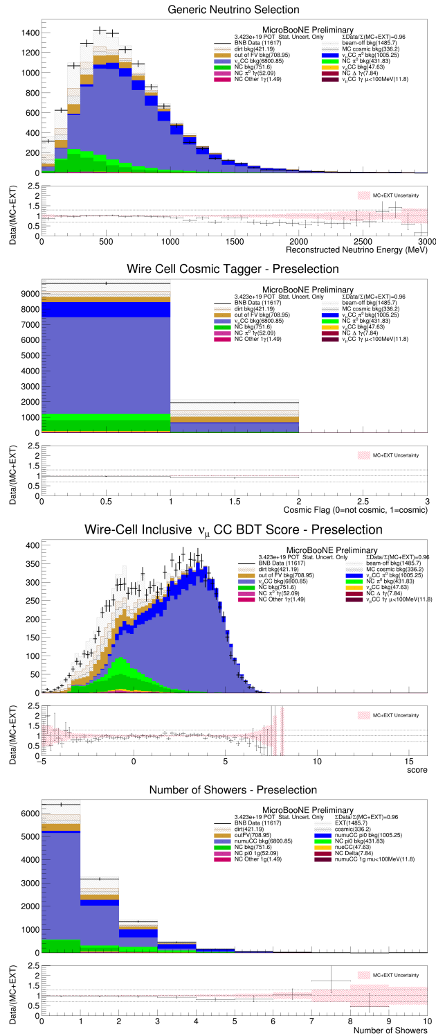
Figure 2: The reconstructed neutrino energy, cosmic tagger flag, Wire-Cell \nu_{\mu} CC BDT score, and number of showers for events immediately after generic neutrino selection. “beam-off” events are cosmic ray events from off-beam data and “MC cosmic” events are simulated neutrino events overlaid on cosmic data where a cosmic induced flash/cluster was selected instead of the neutrino induced one. The data is run 1 open data only, which corresponds to 3.423e19 POT. The middle dashed line on the ratio plots is at \frac{Data}{MC+EXT} = 1 , which indicates exact central value agreement between data and prediction.
