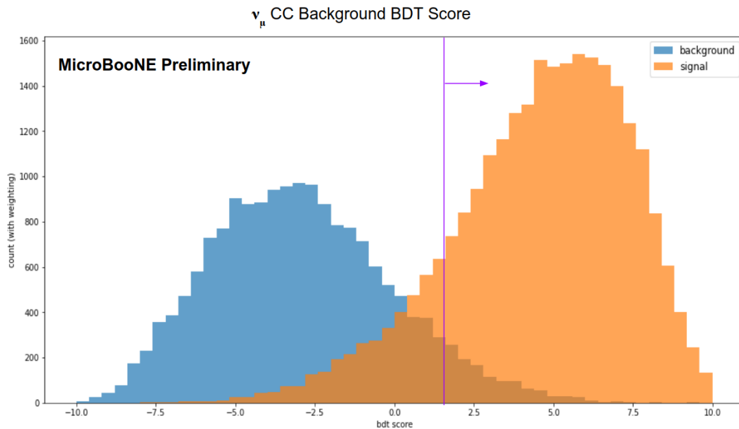
Figure 3: \nu_{\mu} CC background removal BDT scores. Background includes only \nu_{\mu} CC background events. The purple line indicate the cut value for the selection.
