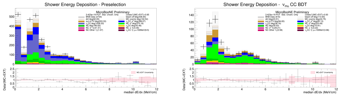
(a) The shower stem dE/dx immediately after preselection - (b) The shower stem dE/dx after preselection and the \nu_\mu CC background BDT cut.
