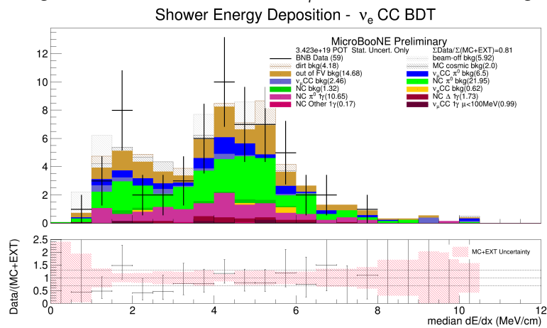
(e) The shower stem dE/dx after preselection and the \nu_\mu CC, other, NC \pi^0 , and \nu_e CC background BDT cuts.
