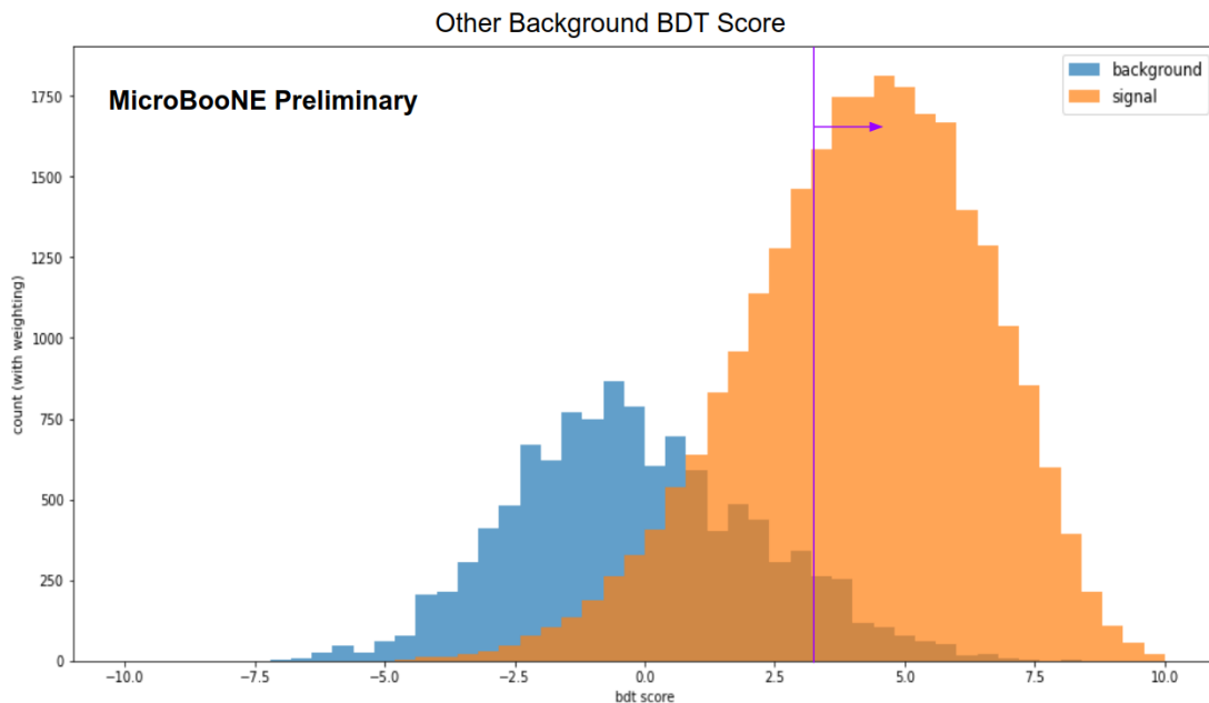
Figure 4: Other background removal BDT scores. Background includes only NC, out of FV, dirt, MC cosmic, and beam-off backgrounds. The purple line indicate the cut value for the selection.
