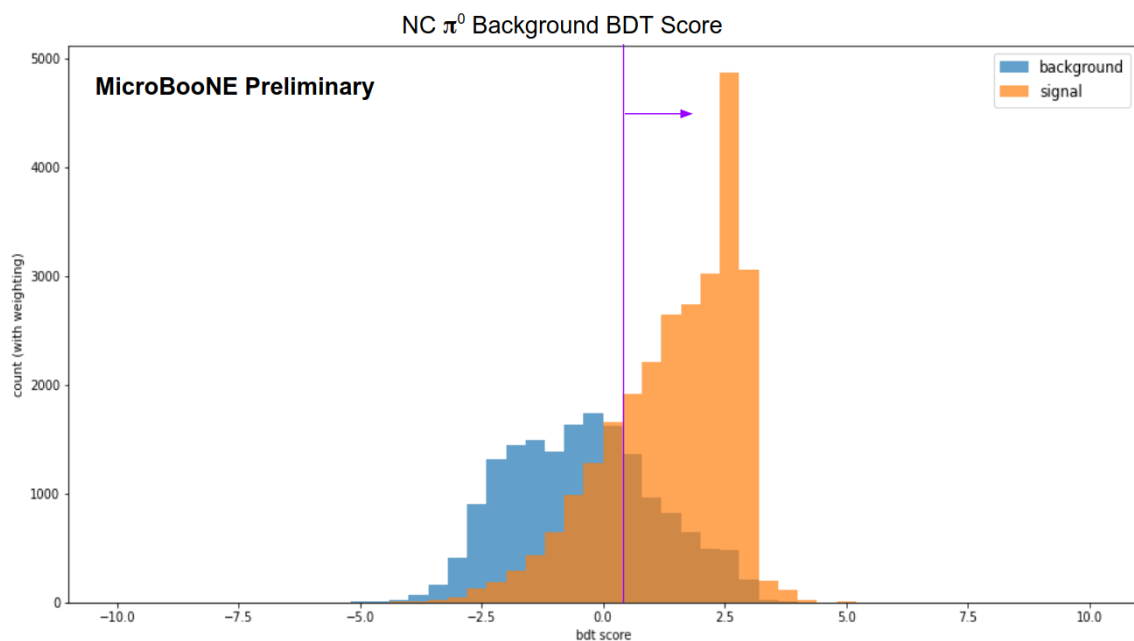
Figure 5: NC \pi^0 background removal BDT scores. Background includes only NC \pi^0 events from BNB overlay and NC \pi^0 overlay. The purple line indicate the cut value for the selection.
