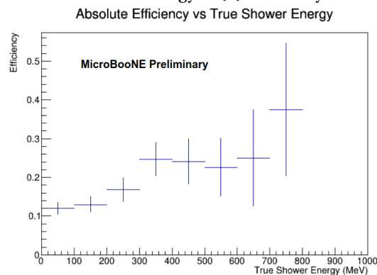
(c) Efficiency as a function of true shower energy.
