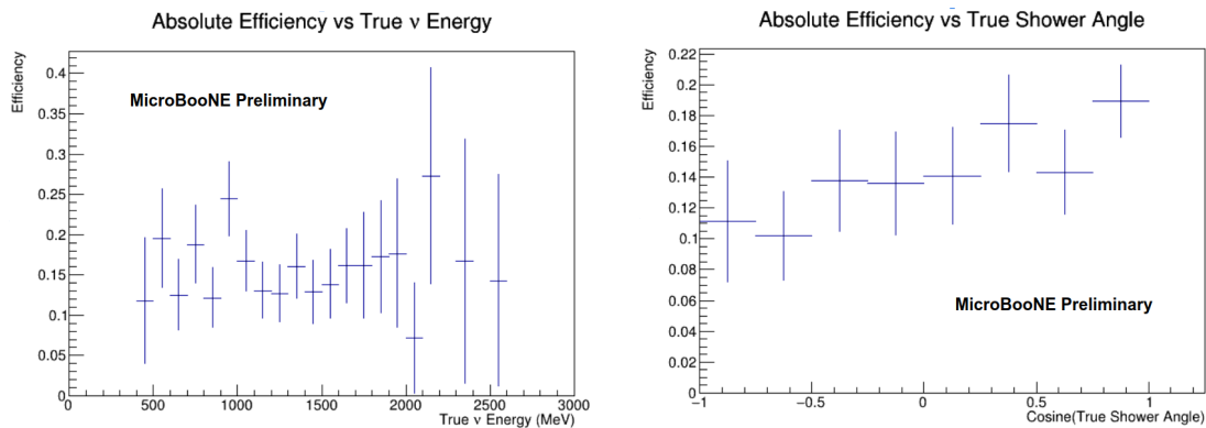
(a) Efficiency as a function of true neutrino energy. (b) Efficiency as a function of true shower angle.
