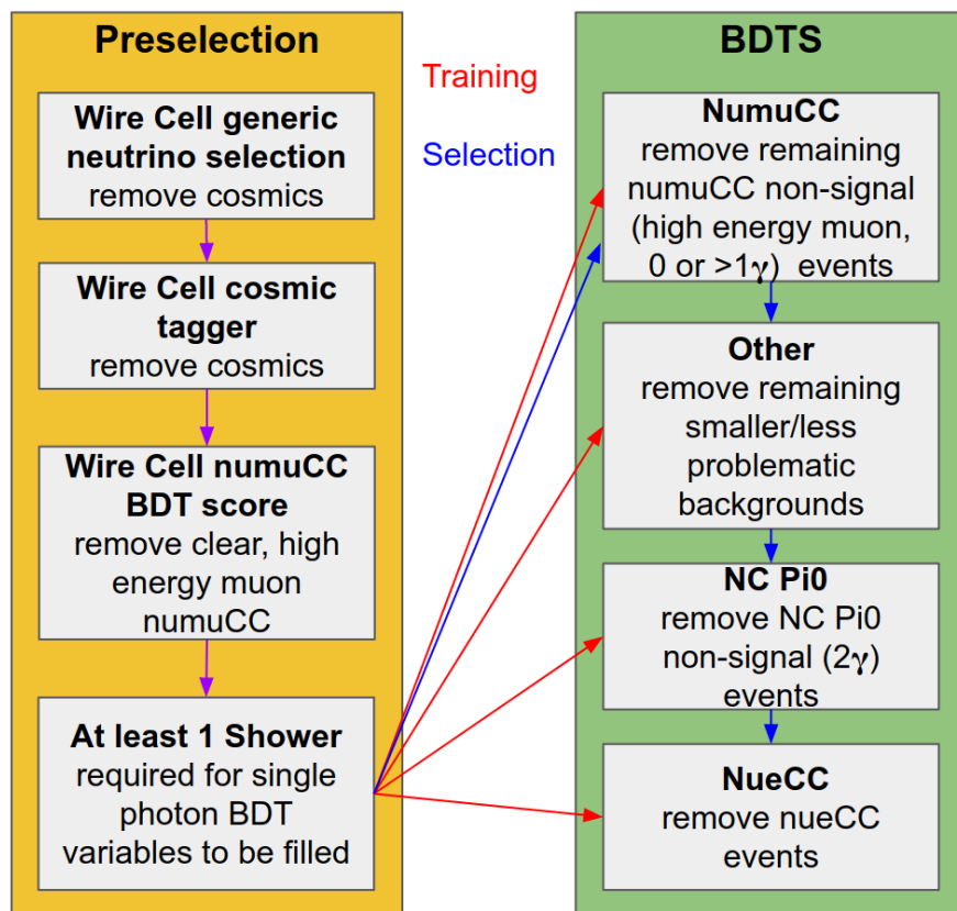
Figure 1: A diagram showing the structure and order of the preselection and BDT training and cuts. The arrows indicate the order of training (red) and selection (blue).
