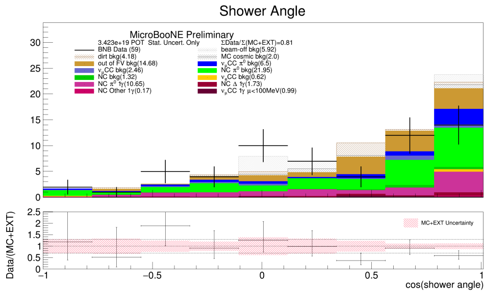
Figure 10: Cosine of reconstructed shower angle with respect to the beam for selected events.
