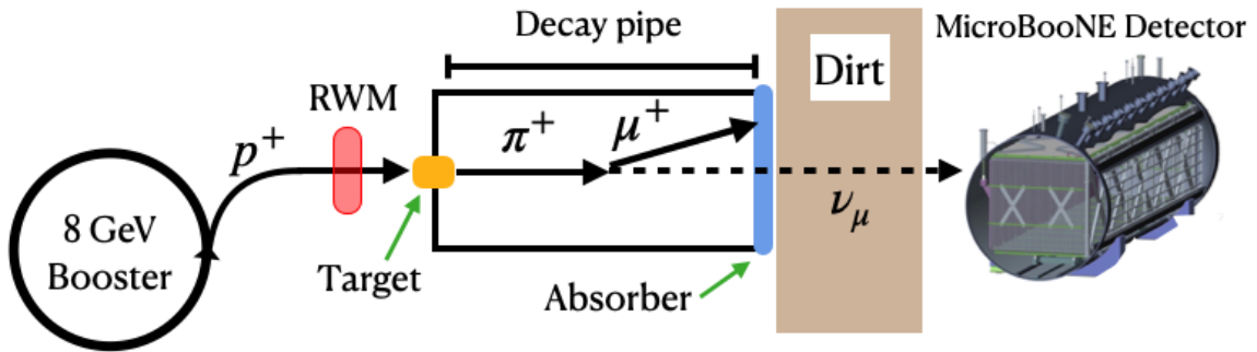
Figure 1: MicroBooNE's detector is in the path of the BNB, on axis with the beam direction, \sim 470 m downstream from the neutrino production target.
